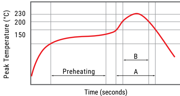
Reflow Profile
