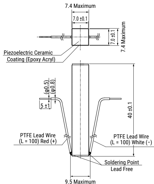
AE0707D44H40DF
