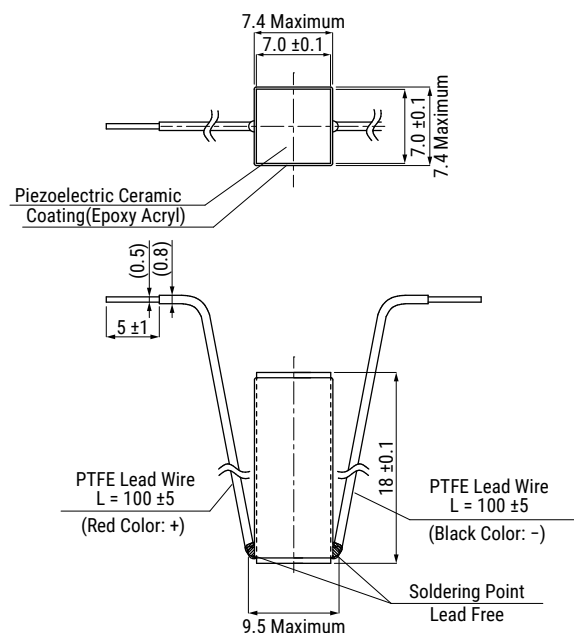
AE0707D18H18DF
