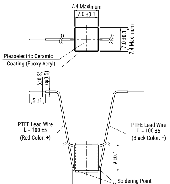
AE0707D08H09DF
