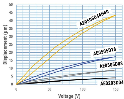
Figure 1 - Voltage vs. Displacement
