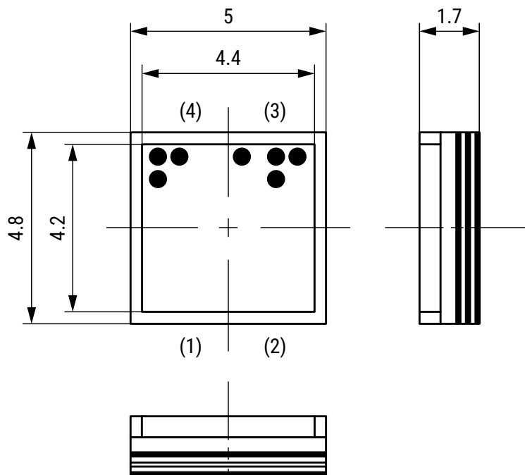
Sensor - Dimensions in mm
